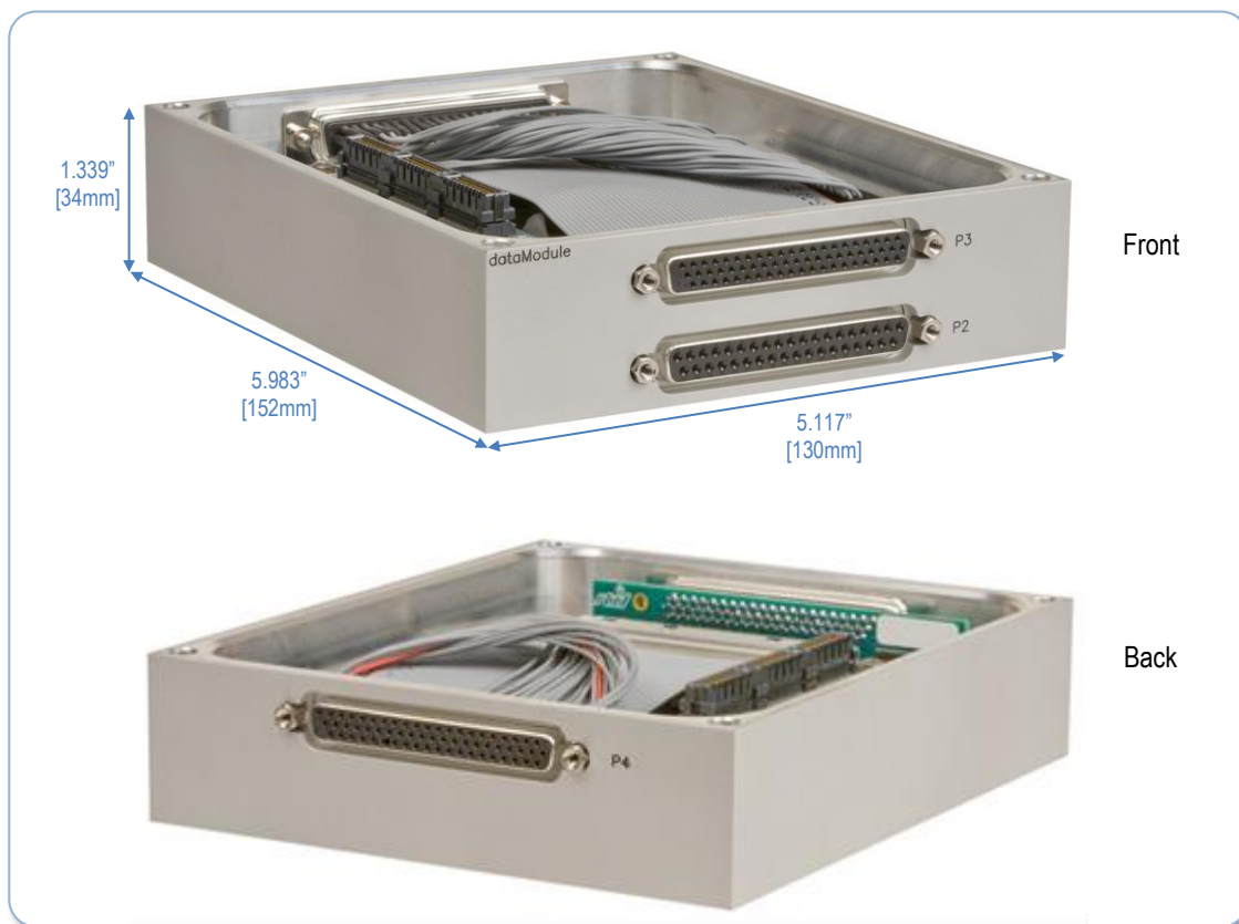
Figure 4: IDAN Dimensions
