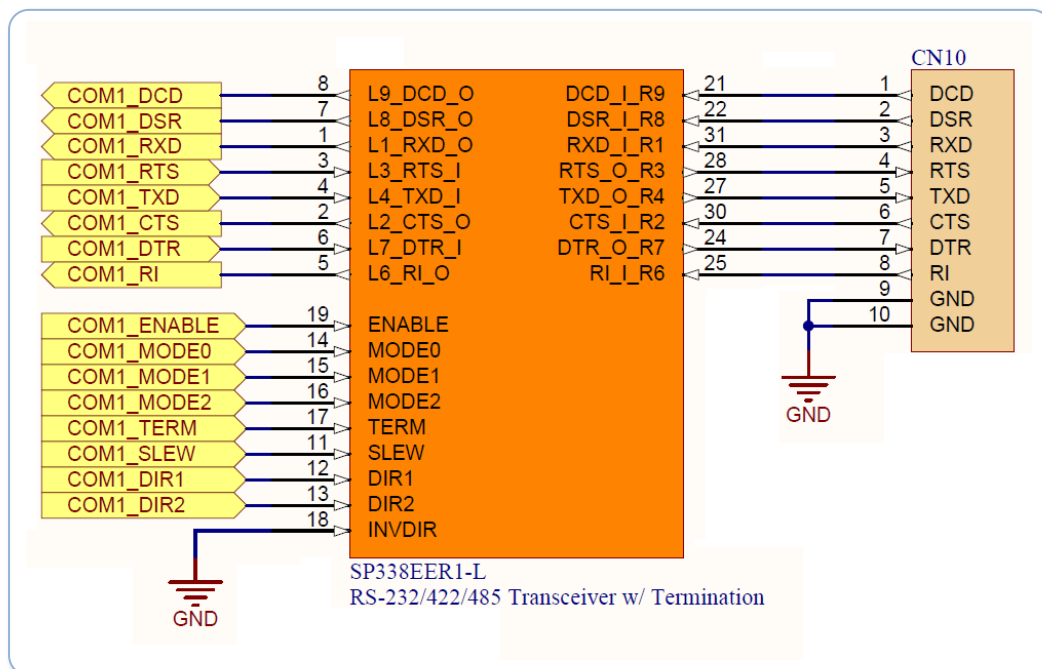
Figure 8: Serial Port Transceiver
